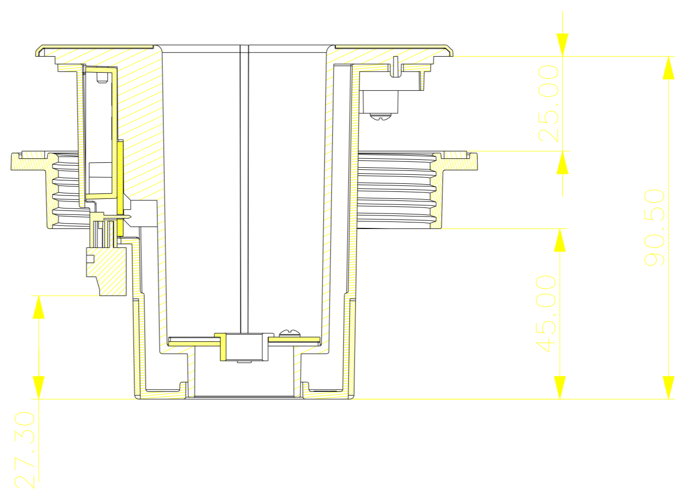
SECTION Y-Y
